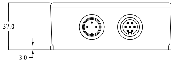
End View
