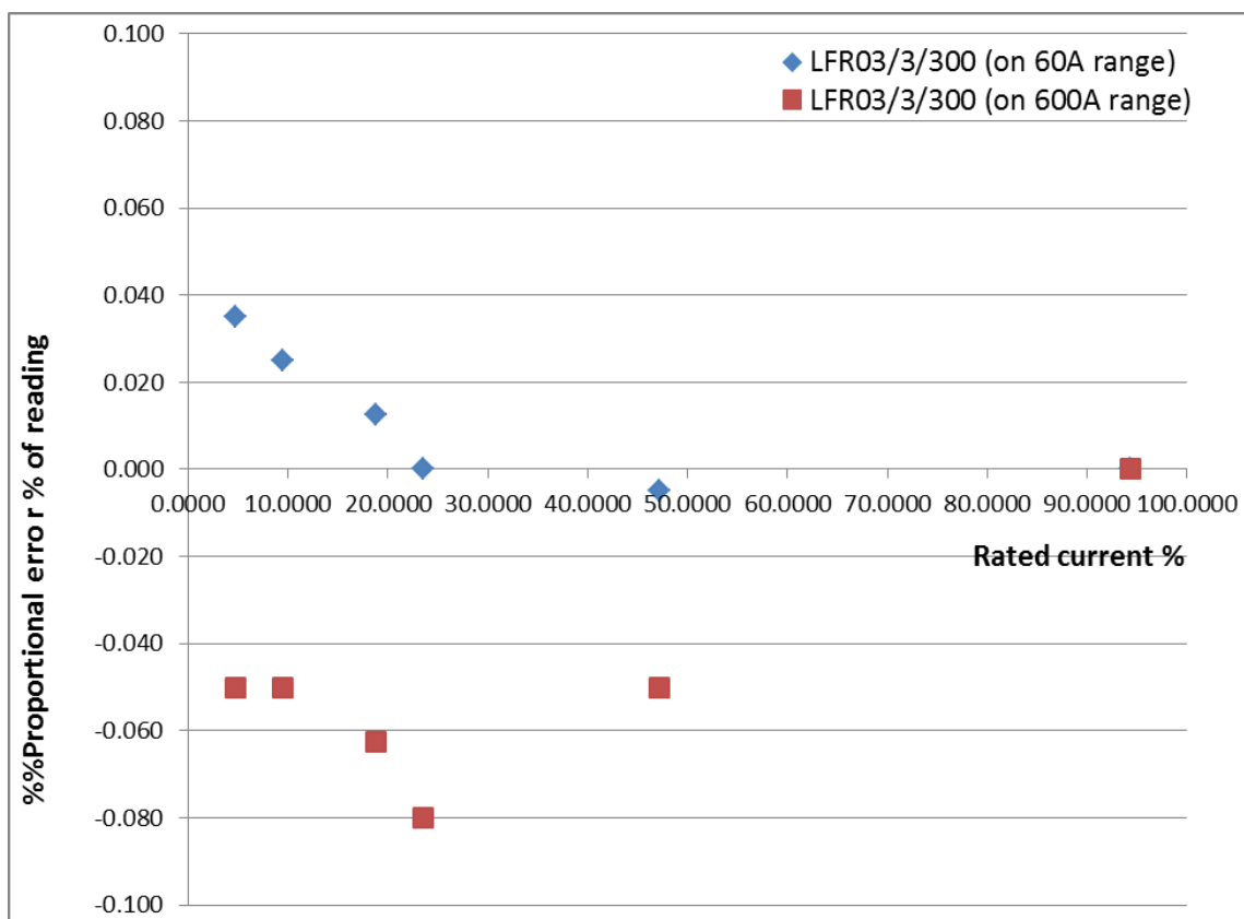
Figure 6. Linearity of the LFR03/3 with 300mm coil
