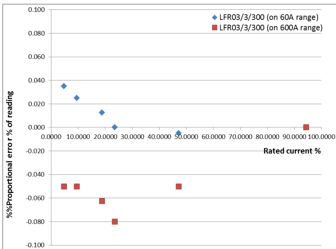
Figure 6. Linearity of the LFR03/3 with 300mm coil
