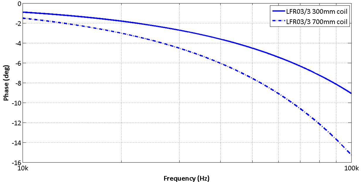
Figure 5. A comparison of phase response 10k to 100kHz the LFR03/3 with a 300mm coil and a 700mm coil.
