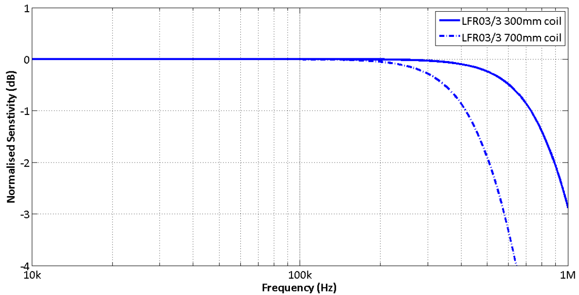
Figure 4. A comparison of the amplitude response > 10kHz of LFR 03/3 with a 300mm coil and a 700mm coil.
