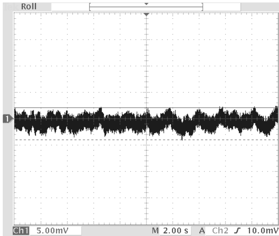
Figure 7. Noise on 10mV/A (600A peak range) LFR03/3 Peak to peak value is 6.1mV corresponding to an rms value of 1.0mV
