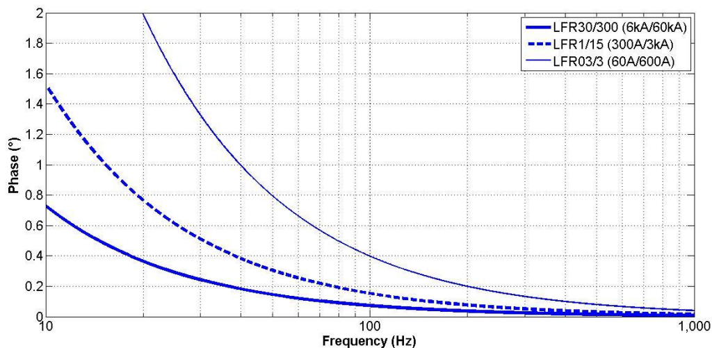
Figure 3. LFR Phase response 10Hz to 1kHz bandwidth
