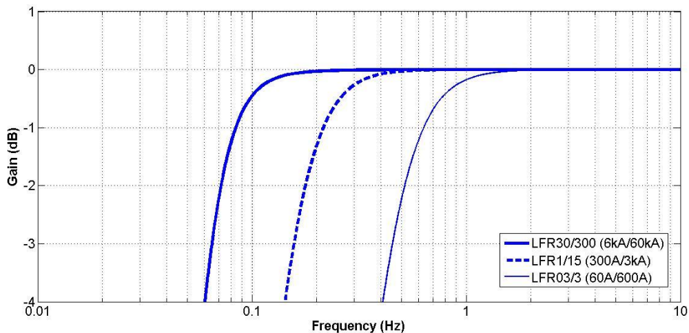
Figure 2. LFR Low frequency (-3dB) bandwidth
