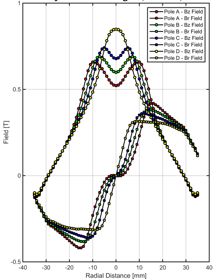
5203 Projected Field Magnet, z=4\text{mm} , I=100\text{A}
