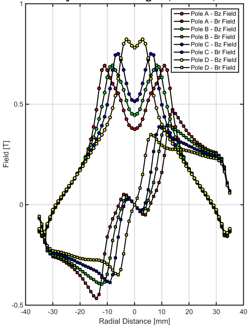
5203 Projected Field Magnet, z=2\text{mm} , I=63\text{A}
