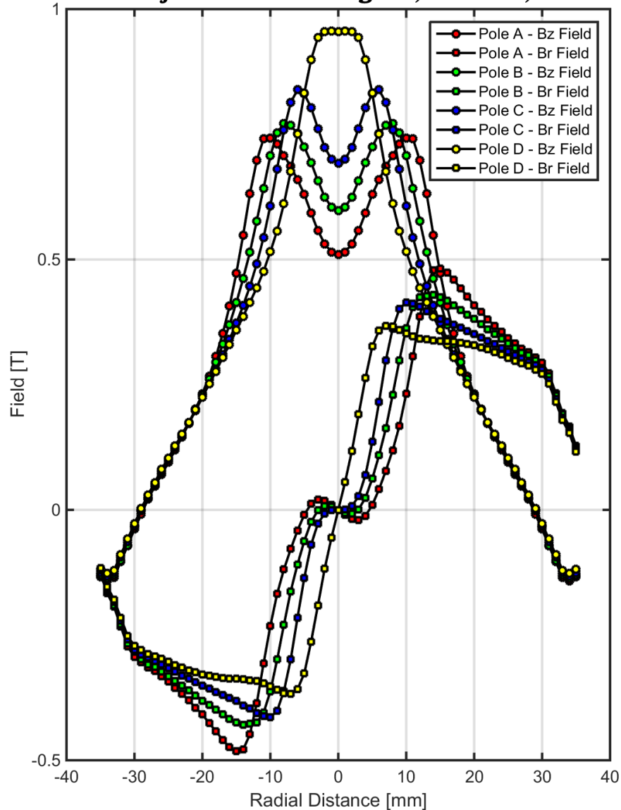
5203 Projected Field Magnet, z=3\text{mm} , I=100\text{A}
