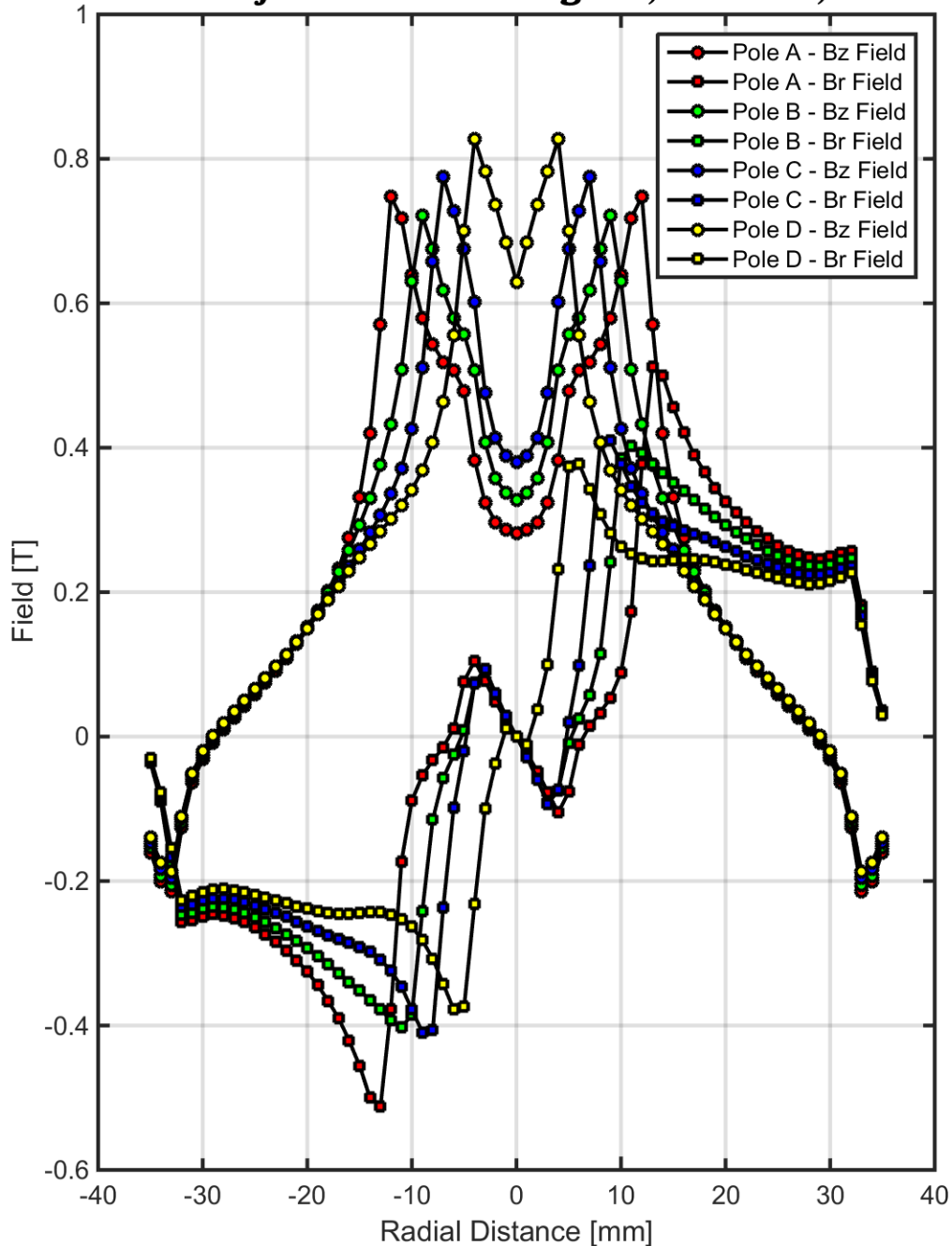
5203 Projected Field Magnet, z=1\text{mm} , I=50\text{A}
