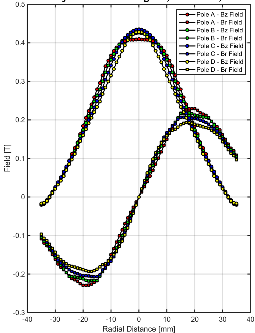
5203 Projected Field Magnet, z=10\text{mm} , I=100\text{A}
