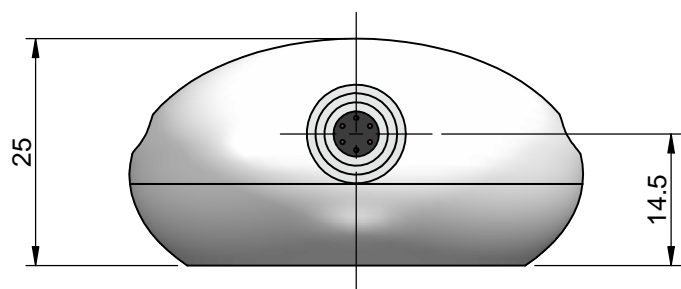
HIROSE HR10-7R-6P(73)
