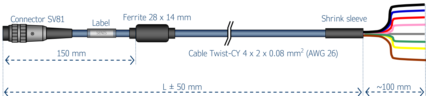
Figure 2. Dimensions and tolerances of the COxx-G signals cable
