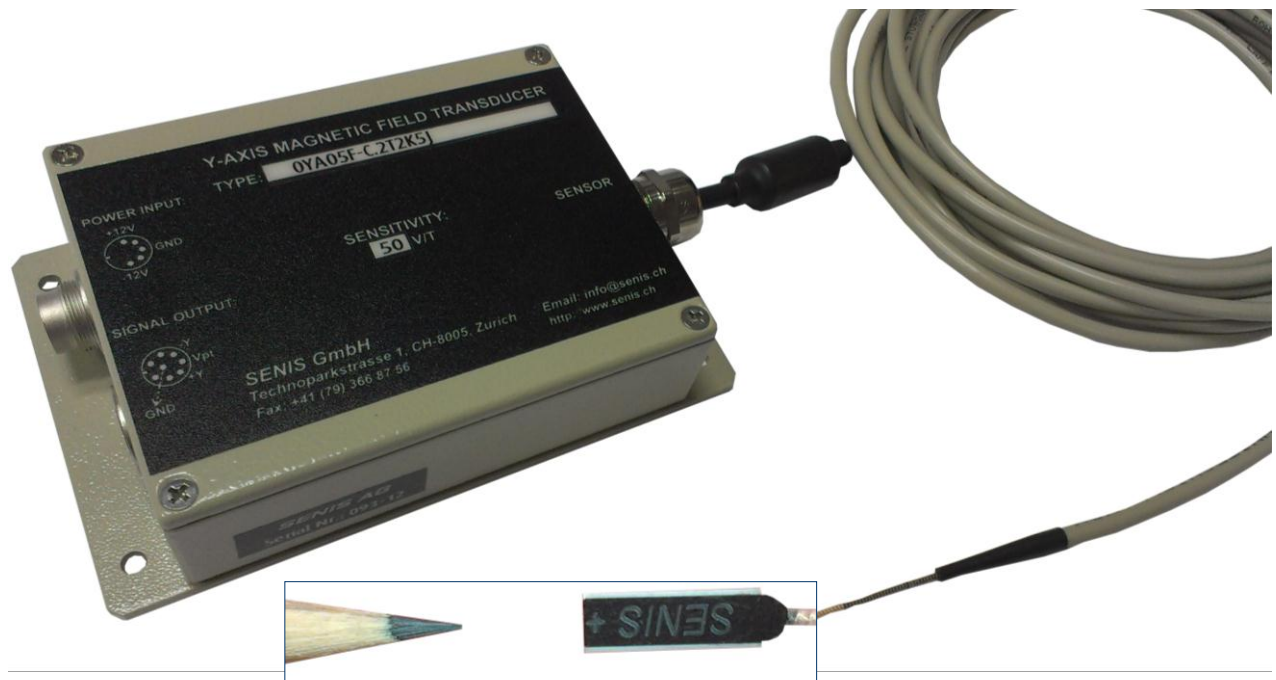
Figure 2. Photo of a 1-axis magnetic field transducer with fully integrated Hall Probe
