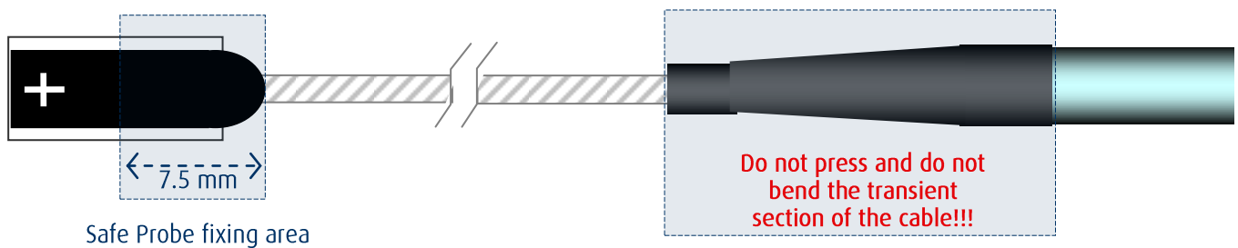
Figure 3. Safe fixing area of the B Probe head
