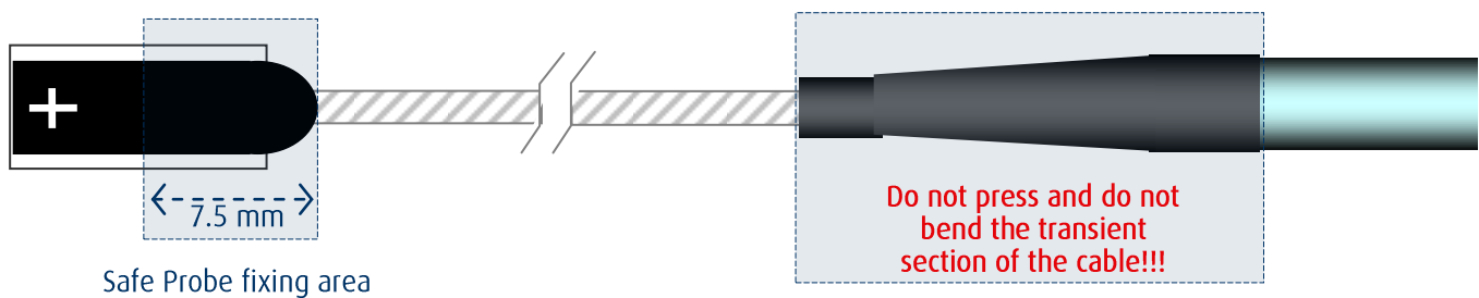
Figure 3. Safe fixing area of the D Probe head
