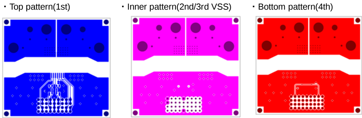
Figure 7. Board layout for measuring thermal resistance of CZ-3703
