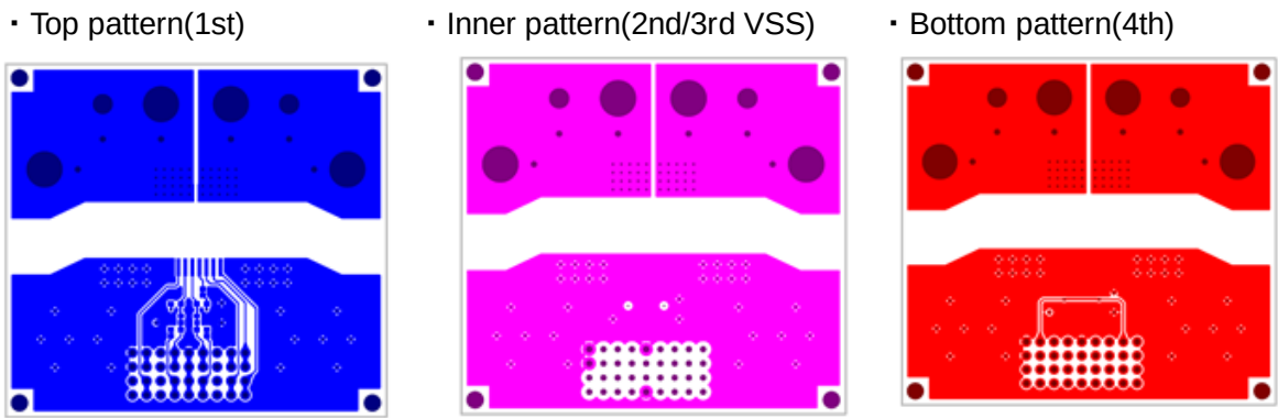
Figure 7. Board layout for measuring thermal resistance of CZ-3705
