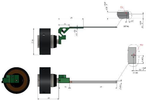
Figure 3: Bend holder with HM probe
